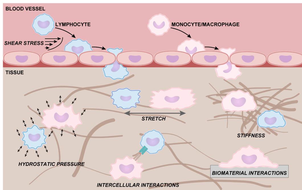
Fig. 1. Common mechanical stimuli experienced by innate and adaptive immune cells. Schematic illustrating the different mechanical stimuli experienced by immune cells as they extravasate through blood vessels and adhere to mechanically active tissues or foreign implantable materials.
