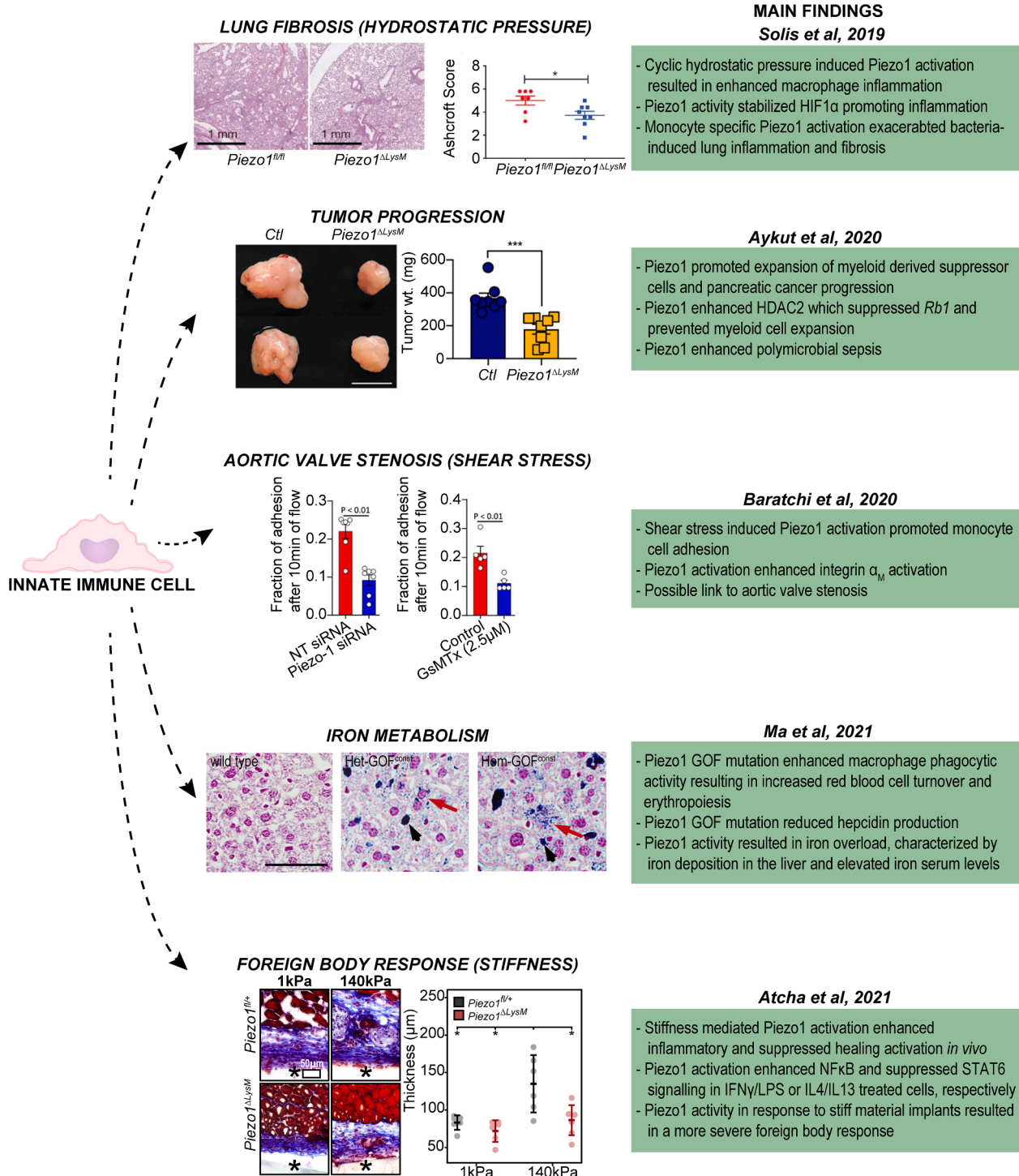
Fig. 3. Piezo1-mediated regulation of innate immune cell function and disease. Summary of recent studies that identify roles for myeloid cell specific Piezo1 in regulating lung fibrosis [85], tumor growth [88], aortic valve stenosis [90], iron metabolism [92], and the foreign body response [61]. Mechanical stimuli identified as key regulators of channel activity are indicated in parentheses. Data shown indicates that myeloid cell specific Piezo1 deletion ( Piezo1 \Delta LysM ) reduced bacteria-induced lung fibrosis, tumor growth, and fibrous encapsulation of stiff implanted materials as is indicated by a reduction in the Ashcroft clinical score, tumor weight, and fibrous capsule thickness, respectively. Moreover, siRNA mediated Piezo1 knockdown or pharmacological inhibition of mechanically-gated ion channels revealed a reduction in monocyte cell adhesion, whereas myeloid cell specific heterozygous (Het-GOF const ) or homozygous (Hom-GOF const ) Piezo1 GOF mutation resulted in enhanced iron deposition in the liver. Arrows indicate presence of iron in hepatocytes.
