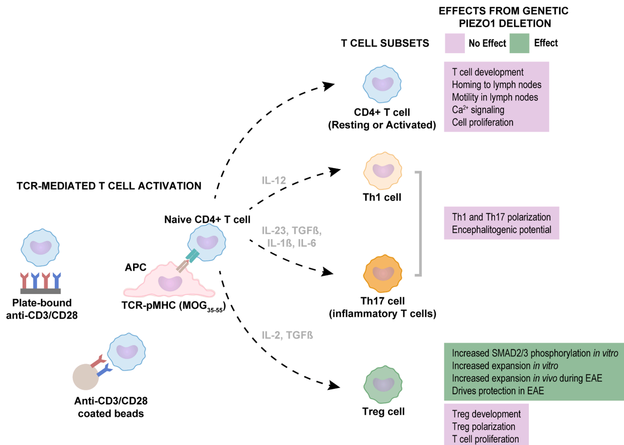
Fig. 4. Effects of Piezo1 deletion in CD4+ T cell subset functions. CD4+ T cells were activated either by peptide recognition on antigen presenting cell (APC) or by TCR-crosslinking antibodies immobilized on beads or a flat-substrate (left). T cell subsets generated by TCR activation in association with specific cytokine cocktails as indicated. Panel on the right shows the effects of Piezo1 deletion in various subsets (see text for details) [113].
